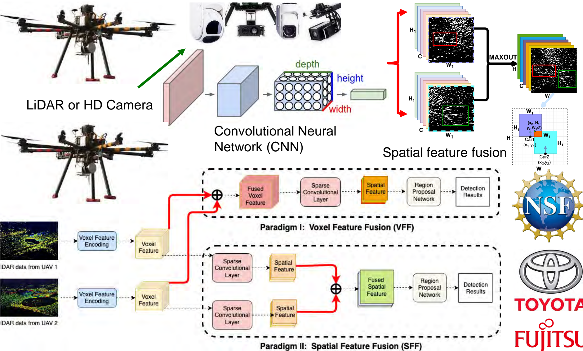
Architecture of the feature based cooperative perception (F-Cooper)
