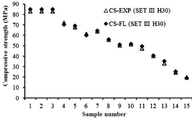
13 Matching figure of results of CS for SET III H30 (FL versus EXP)
