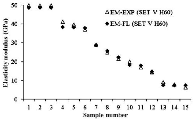
16 Matching figure of results of EM for SET V H60 (FL versus EXP)
