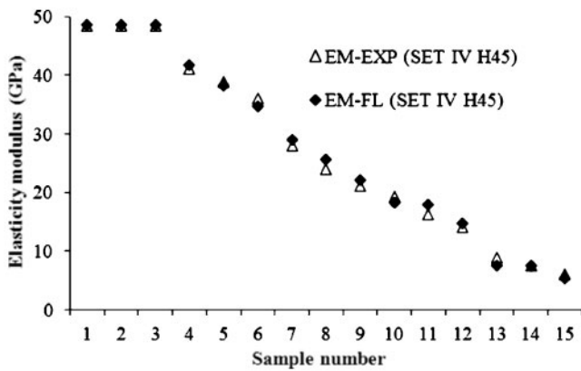
14 Matching figure of results of EM for SET IV H45 (FL versus EXP)
