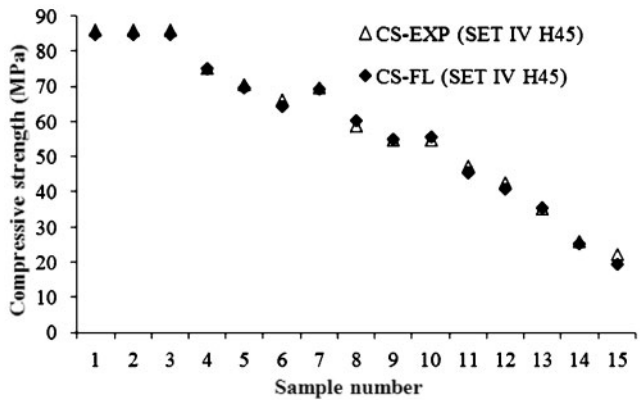
15 Matching figure of results of CS for SET IV H45 (FL versus EXP)
