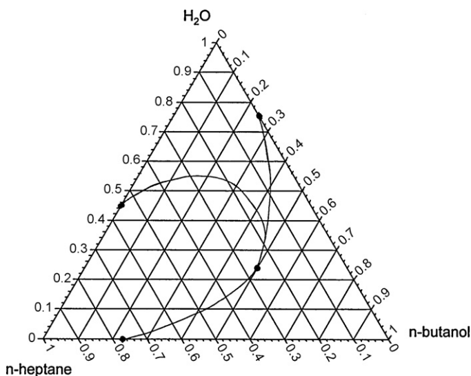
Fig. 1. Binary and ternary azeotropes and approximate valley lines on the normal boiling temperature surface in the system water + n-heptane + 1-butanol.
