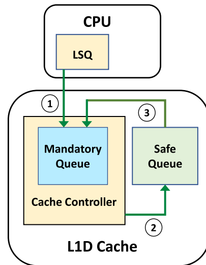
Fig. 5. SafeLoadOnMiss design.
